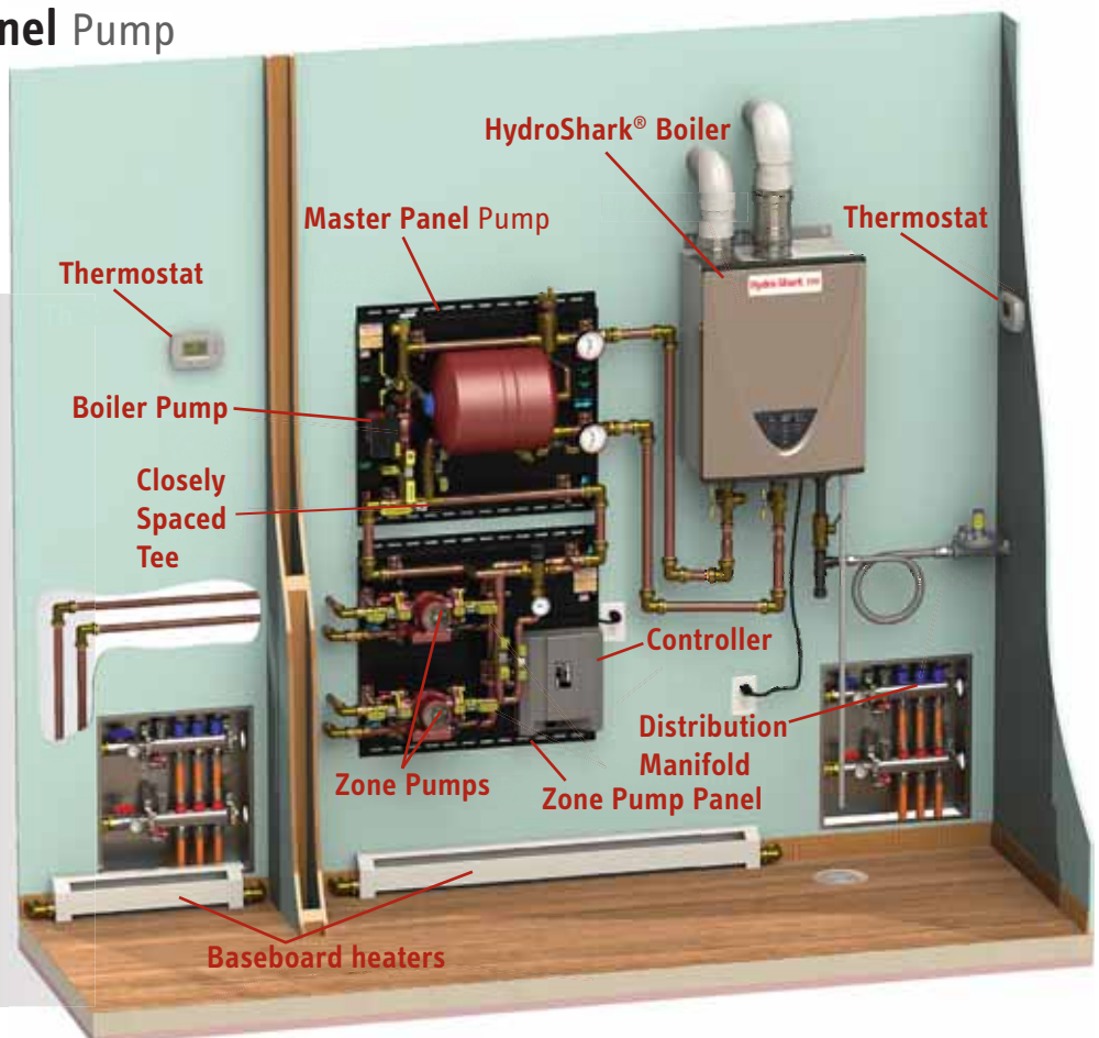
Shown: Master Panel Pump, 2-Zone Pump Panel, HydroShark 199
